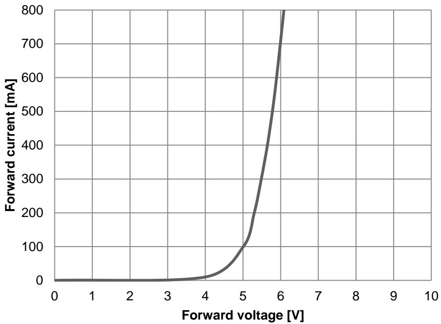
Fig 2. Forward Voltage vs. Forward Current, T_a=25^\circ\text{C}
