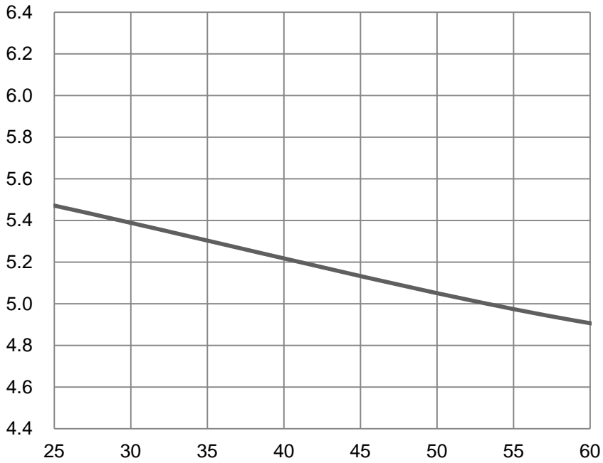
Fig 7. Ambient Temperature vs. Forward Voltage, I_F=600\text{mA}
