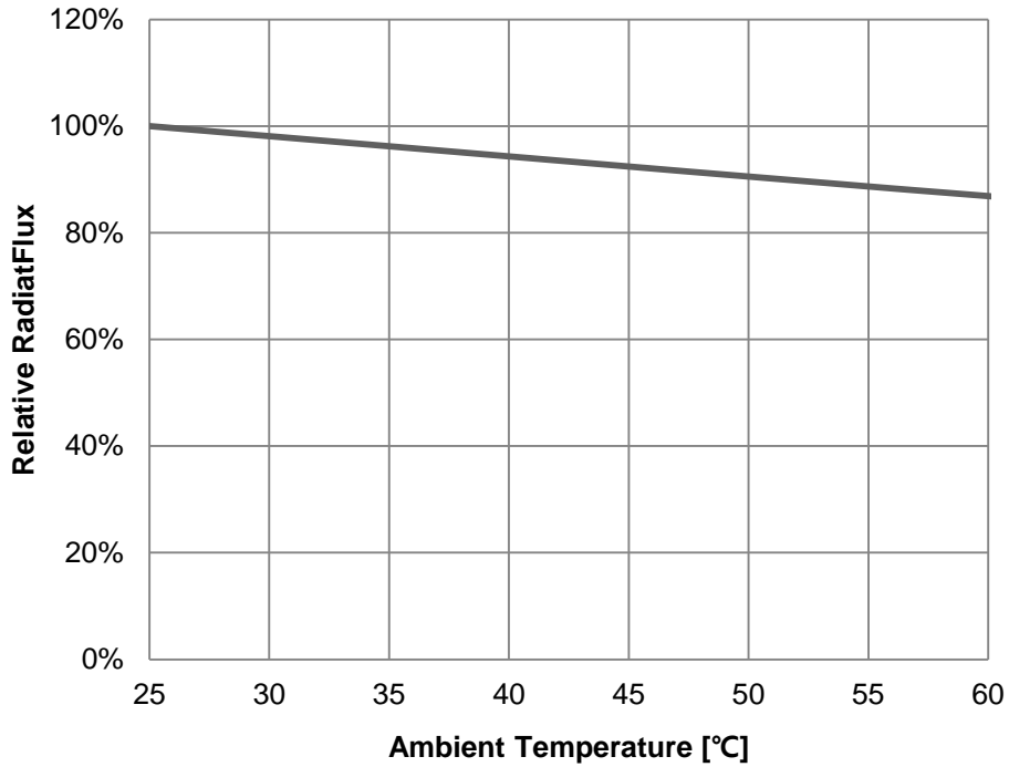
Fig 5. Ambient Temperature vs. Relative Radiant Flux, I_F=600mA
