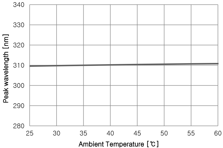
Fig 6. Ambient Temperature vs. Peak Wavelength, I_F=600mA
