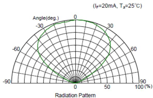
Radiation Pattern
