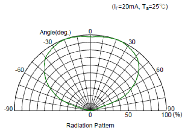
Radiation Pattern
