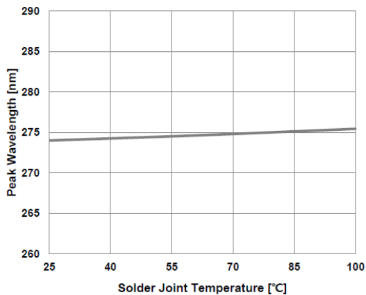
Peak Wavelength vs. Solder Joint Temp.
