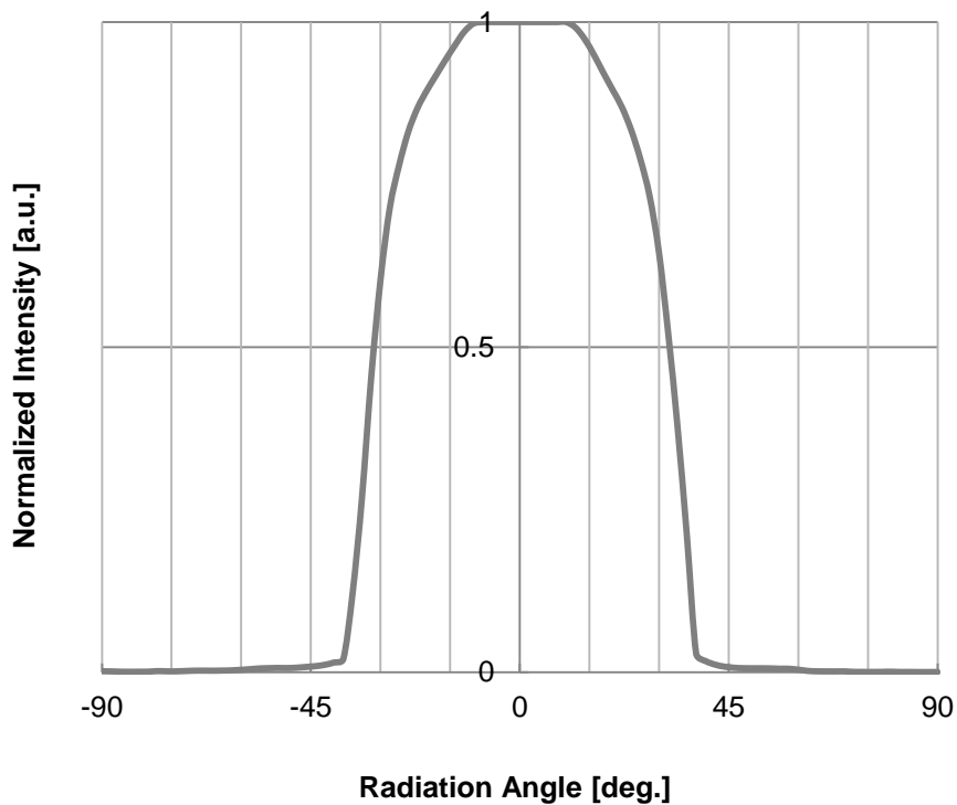
Fig 8. Typical Spatial Distribution, I_F=1A
