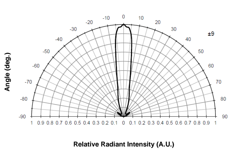
Radiation Characteristics
