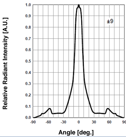
Radiation Characteristics
