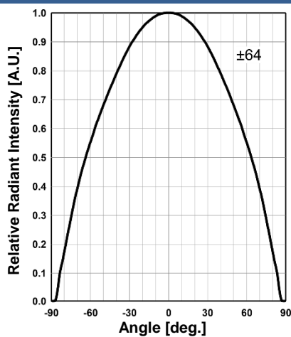
Radiation Characteristics
